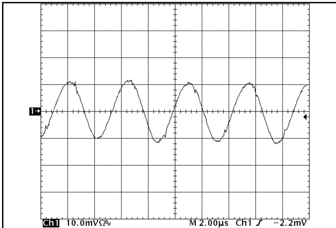
Figure 19: Input reflected ripple current, i_s , through a 10\ \mu\text{H} source inductor at nominal input voltage and rated load current ( 10\ \text{mA}/\text{div} ). See Figure 17.
