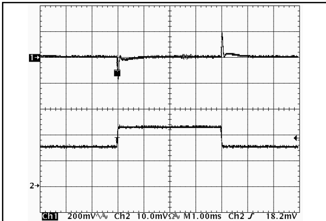
Figure 15: Output voltage response to step-change in load current (50%-75%-50% of Iout(max); dI/dt = 0.1A/\mu s ). Load cap: 10 \mu F , 100 m \Omega ESR tantalum cap and 1 \mu F ceramic cap. Ch 1: Vout (200mV/div), Ch 2: Iout (10A/div).
