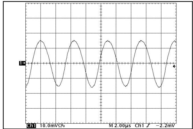
Figure 18: Input Terminal Ripple Current, i_c , at full rated output current and nominal input voltage with 10\ \mu\text{H} source impedance and 47\ \mu\text{F} electrolytic capacitor ( 500\ \text{mA}/\text{div} ). See Figure 17.
