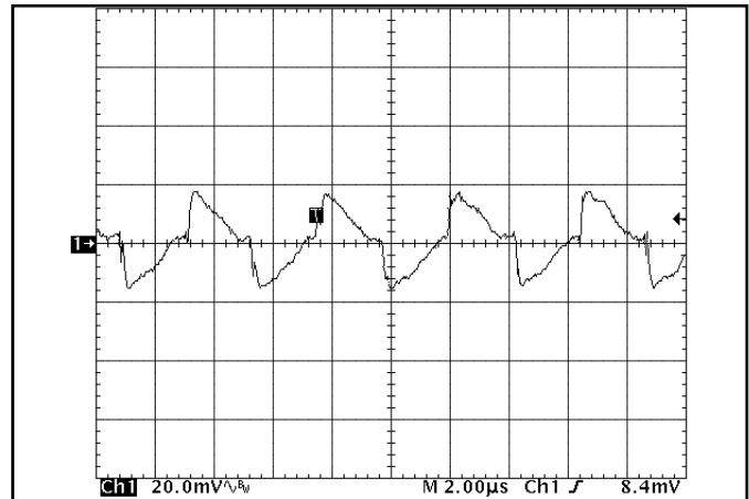
Figure 20: Output voltage ripple at nominal input voltage and rated load current ( 20\ \text{mV}/\text{div} ). Load capacitance: 1\ \mu\text{F} ceramic capacitor and 10\ \mu\text{F} tantalum capacitor. Bandwidth: 20\ \text{MHz} . See Figure 17.
