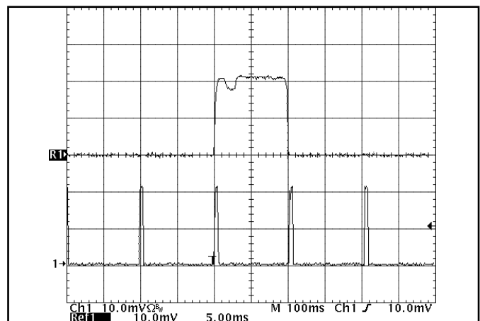
Figure 22: Load current ( 20\text{A}/\text{div} ) as a function of time when the converter attempts to turn on into a 10\ \text{m}\Omega short circuit. Top trace ( 5\text{ms}/\text{div} ) is an expansion of the on-time portion of the bottom trace.
